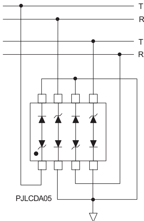
Ethernet Application
