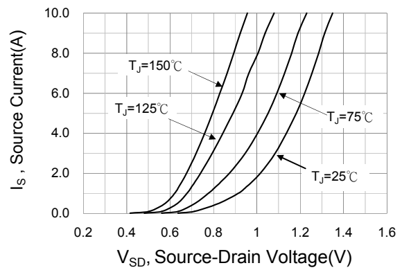
Fig.8 Body diode forward voltage
