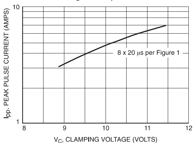
Figure 4. Clamping Voltage versus Peak Pulse Current
