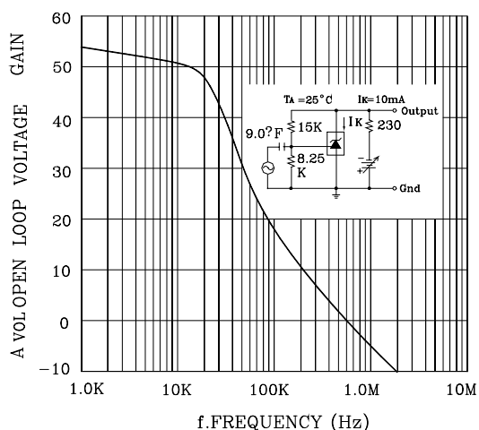
FIGURE 12 - OPEN LOOP VOLTAGE GAIN VERSUS FREQUENCY
