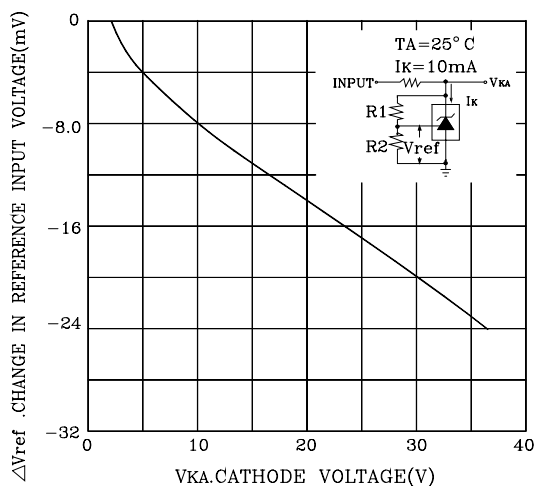
FIGURE 8-CHANGE IN REFERENCE INPUT VOLTAGE versus CATHODE VOLTAGE
