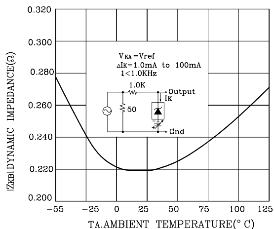
FIGURE 11 - DYNAMIC IMPEDANCE VERSUS AMBIENT TEMPERATURE
