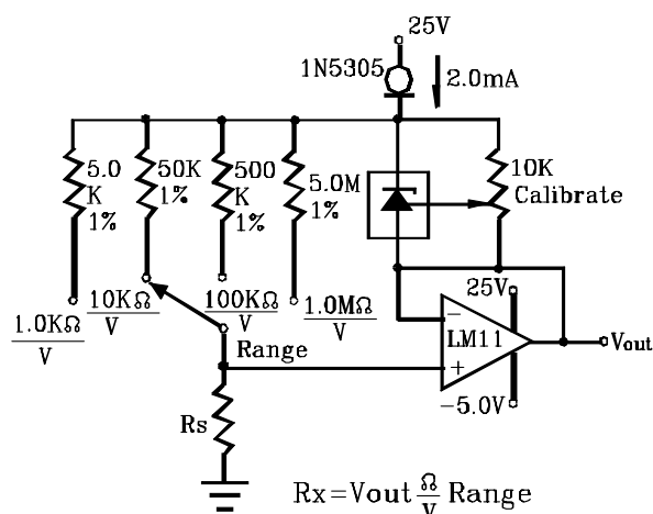
FIGURE 28-LINER OHMMETER
