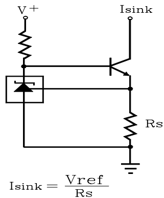
FIGURE 23-CONSTANT CURRENT SINK
