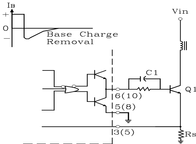
FIGURE 28-BIPOLAR TRANSISTOR DRIVE
