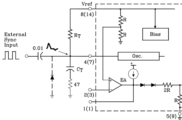
FIGURE 20-EXTERNAL CLOCK SYNCHRONIZATION
