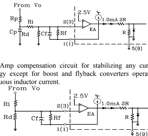
FIGURE 31-ERROR AMPLIFIER COMPENSATION
