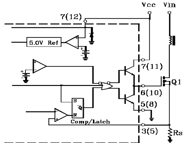
FIGURE 27-MOSFET PARASITIC OSCILLATIONS
