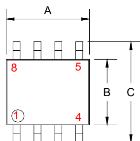
1.Top View
