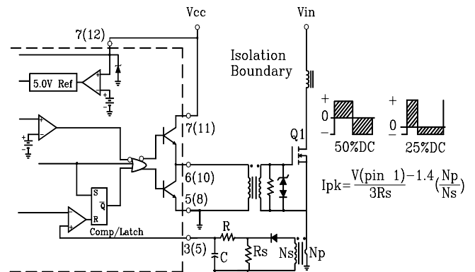
FIGURE 29-ISOLATED MOSFET DRIVE
