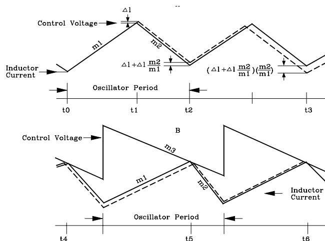
FIGURE 19-CONTINUOUS CURRENT WAVEFORMS
