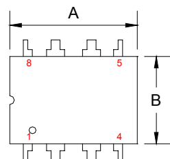
1.Top View
