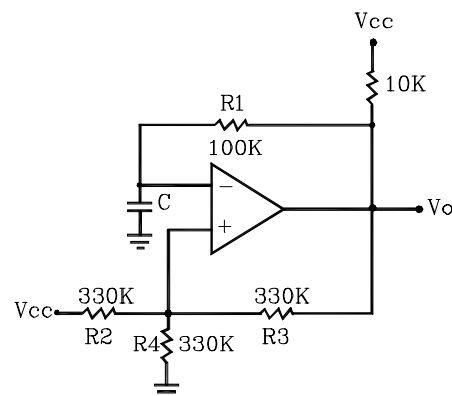
FIGURE 8 - SQUAREWAVE OSCILLATOR
