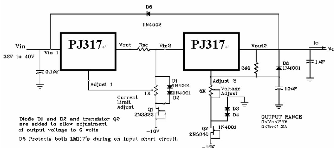
FIGURE 20-ADJUSTABLE CURRENT LIMITER
