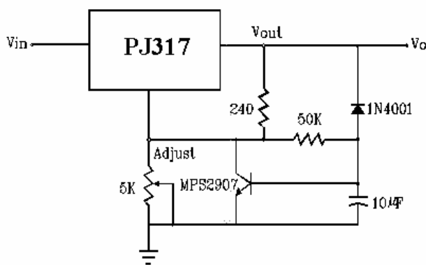
FIGURE 22-SLOW TURN-ON REGULATOR
