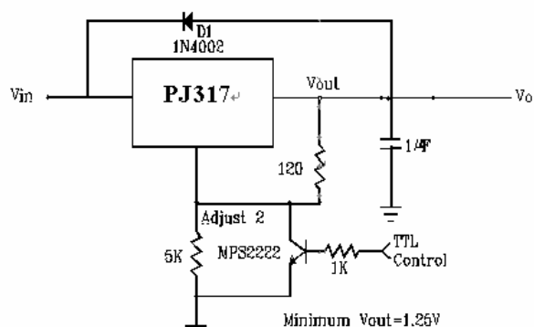
FIGURE 21-5V ELECTRONIC SHUT DOWN REGULATOR
