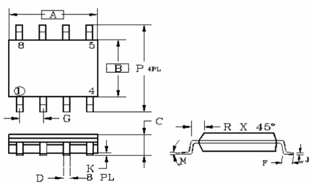
SOP-8
