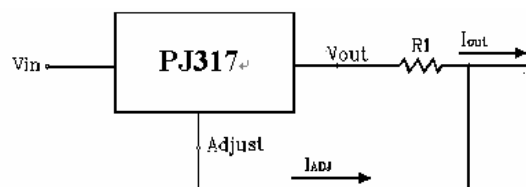
FIGURE 23-CURRENT REGULATOR
