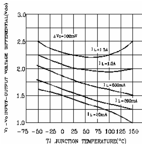
FIGURE 8-DROPOUT VOLTAGE
