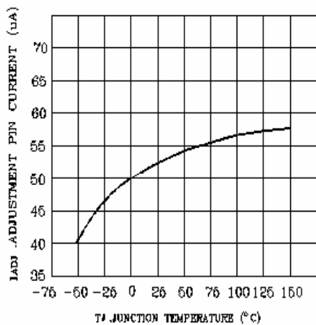
FIGURE 9-TEMPERATURE STABILITY CURRENT
