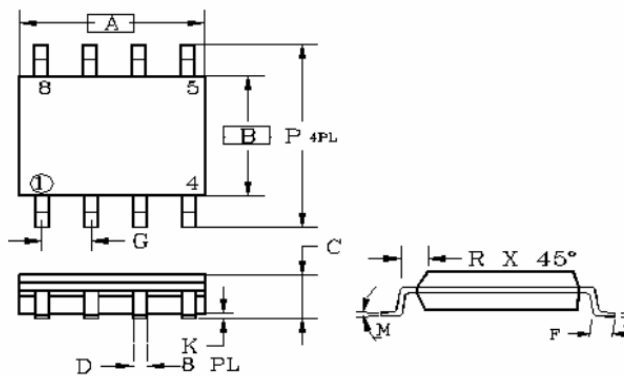
SOP-8
