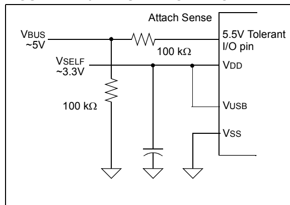
FIGURE 22-10: SELF-POWER ONLY
