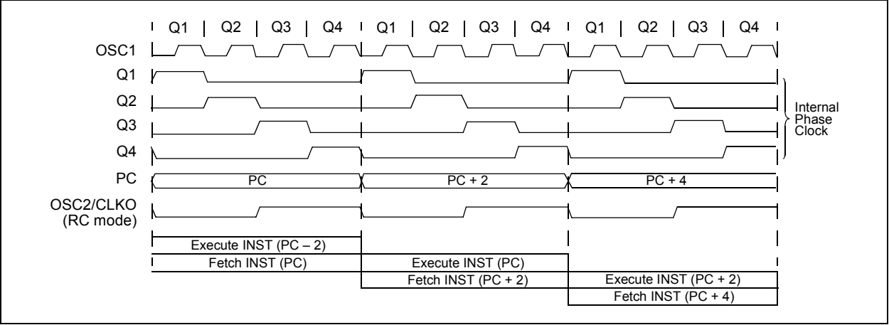
FIGURE 5-5: CLOCK/INSTRUCTION CYCLE
