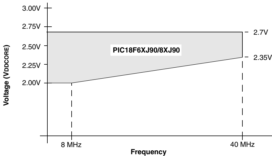
FIGURE 25-2: PIC18F85J90 FAMILY VOLTAGE-FREQUENCY GRAPH, REGULATOR DISABLED (INDUSTRIAL) (1,2)
