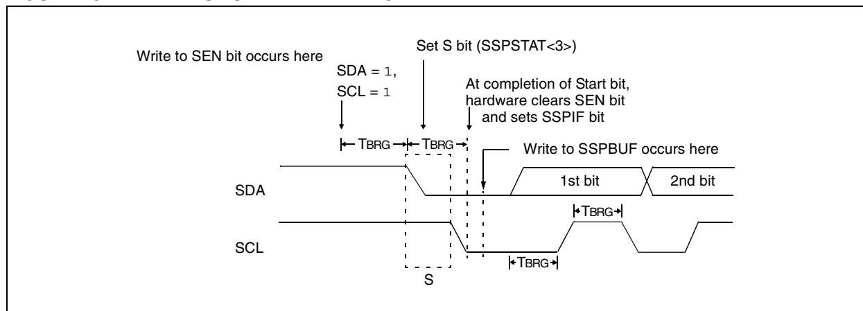
FIGURE 16-21: FIRST START BIT TIMING
