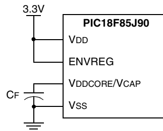
FIGURE 22-2: CONNECTIONS FOR THE ON-CHIP REGULATOR
