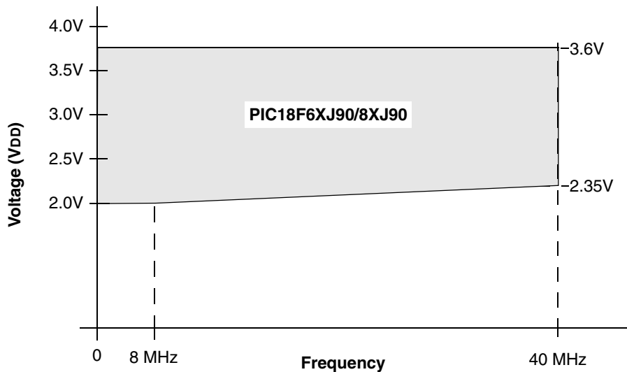
FIGURE 25-1: PIC18F85J90 FAMILY VOLTAGE-FREQUENCY GRAPH, REGULATOR ENABLED (INDUSTRIAL) (1)
