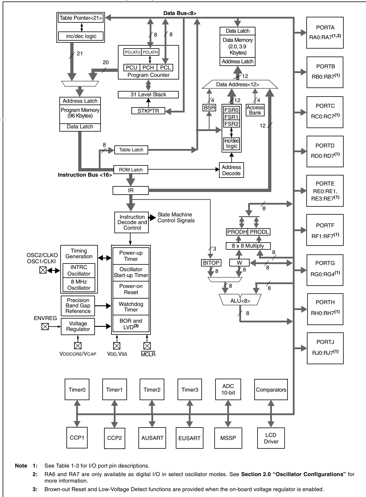
FIGURE 1-2: PIC18F8XJ90 (80-PIN) BLOCK DIAGRAM
