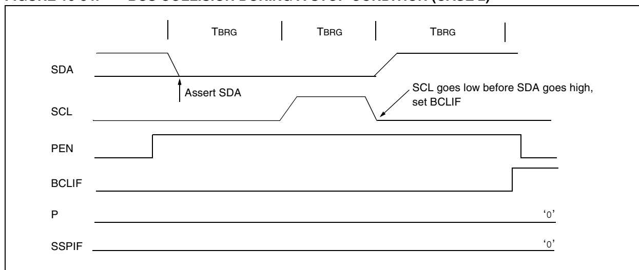
FIGURE 16-34: BUS COLLISION DURING A STOP CONDITION (CASE 2)
