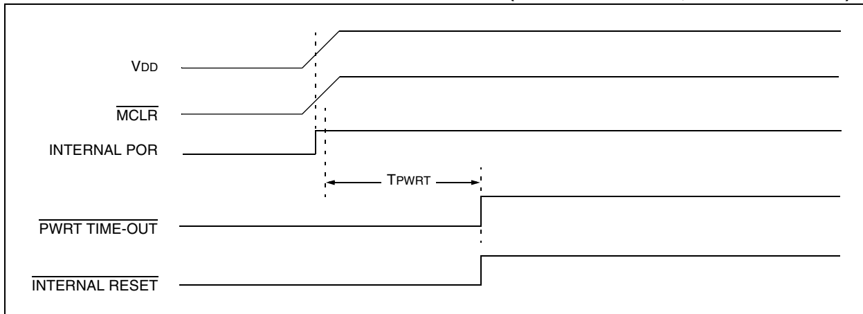
FIGURE 4-3: TIME-OUT SEQUENCE ON POWER-UP ( \overline{\text{MCLR}} TIED TO V_{\text{DD}} , V_{\text{DD}} \text{ RISE} < T_{\text{PWRT}} )
