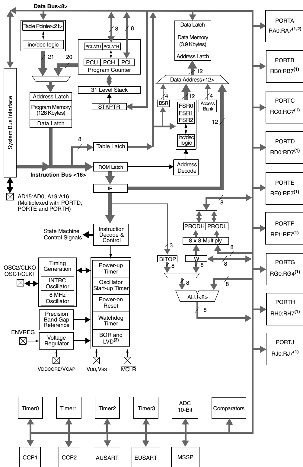
FIGURE 1-2: PIC18F8XJ11 (80-PIN) BLOCK DIAGRAM
