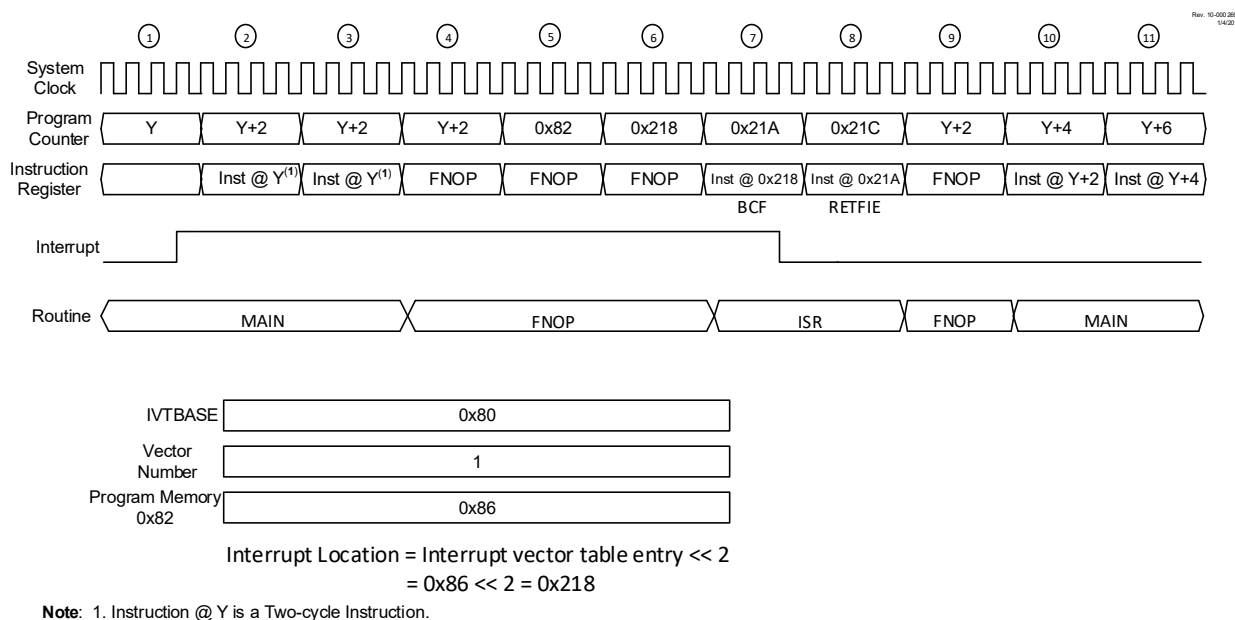
Figure 11-8. Interrupt Timing Diagram: Two-Cycle Instruction
