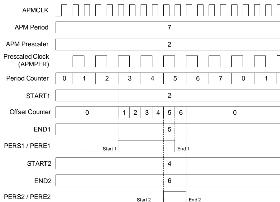
Figure 18-1. Analog Peripheral Manager Timing Diagram (APMPRE = 2 and APMPER = 7)
