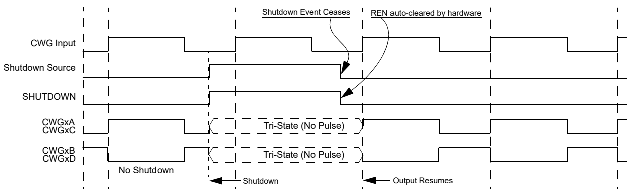
Figure 33-16. Shutdown Functionality, Auto-Restart Enabled (REN = 1, LSAC = 'b01, LSB = 'b01)
