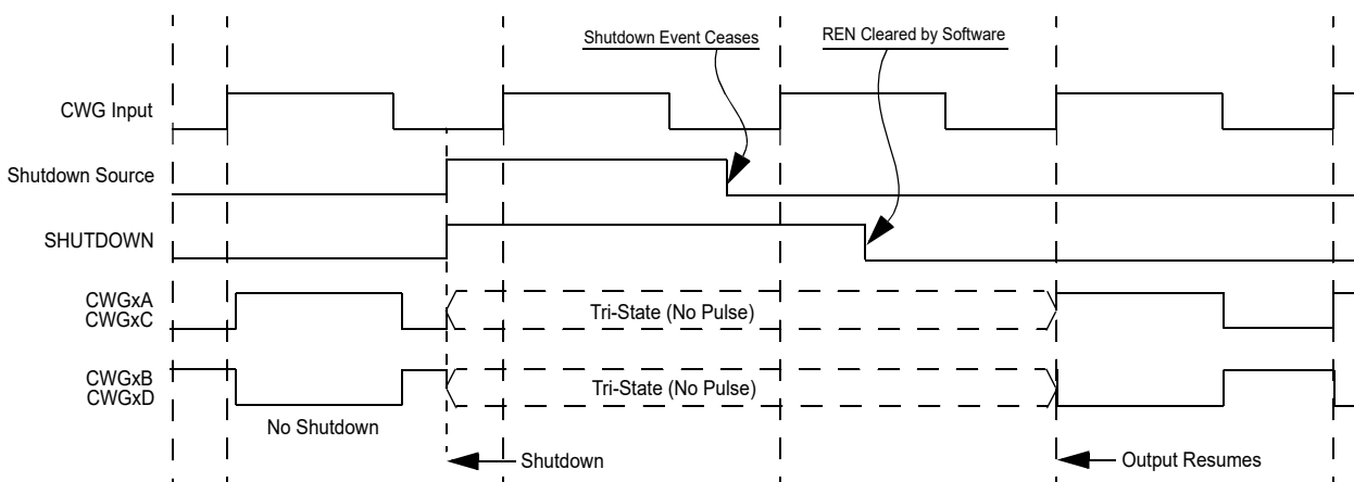
Figure 33-15. Shutdown Functionality, Auto-Restart Disabled (REN = 0, LSAC = 'b01, LSB = 'b01)
