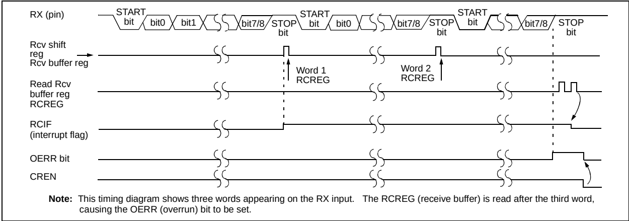
FIGURE 16-5: ASYNCHRONOUS RECEPTION
