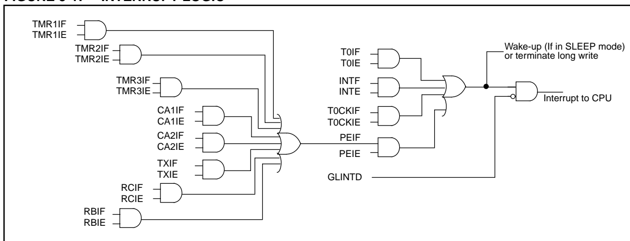
FIGURE 5-1: INTERRUPT LOGIC
