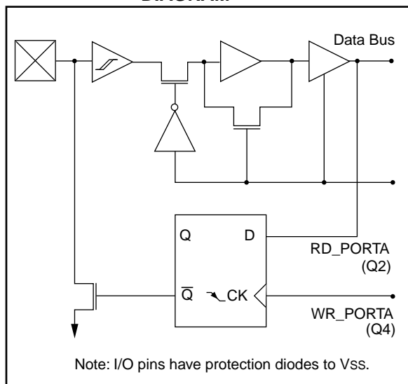
FIGURE 9-2: RA2 AND RA3 BLOCK DIAGRAM
