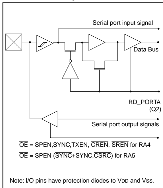
FIGURE 9-3: RA4 AND RA5 BLOCK DIAGRAM
