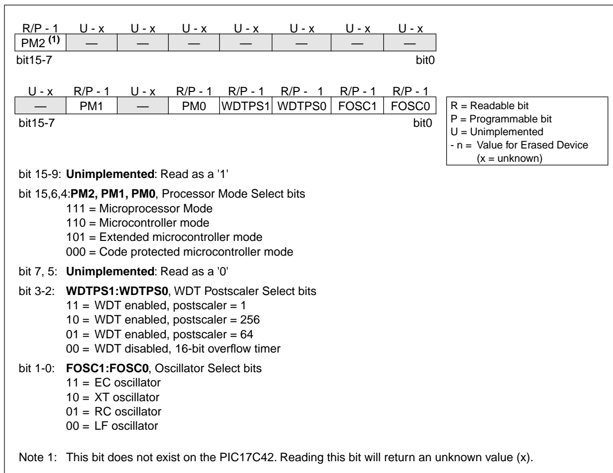
FIGURE 14-1: CONFIGURATION WORD
