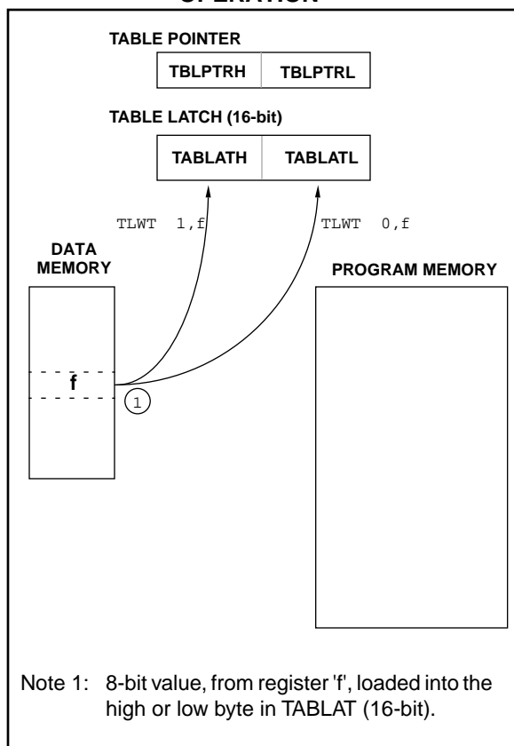
FIGURE 7-1: TLWT INSTRUCTION OPERATION
