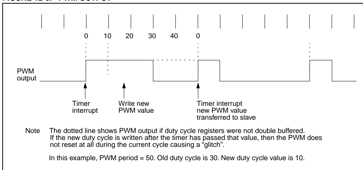
FIGURE 12-6: PWM OUTPUT
