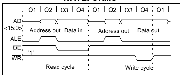
FIGURE 6-3: EXTERNAL PROGRAM MEMORY ACCESS WAVEFORMS
