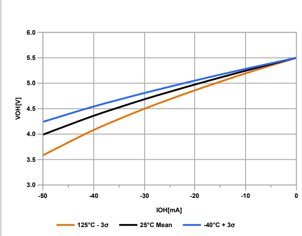
Figure 33-36. V_{OH} vs. I_{OH} OVER TEMPERATURE, V_{DD} = 5.5\text{V}
