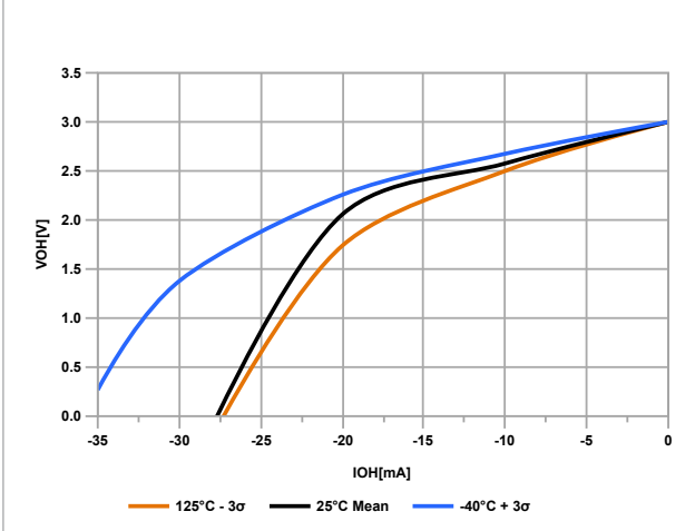
Figure 33-37. V_{OH} vs. I_{OH} OVER TEMPERATURE, V_{DD} = 3\text{V}
