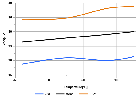
Figure 33-9. BROWN-OUT RESET HYSTERESIS, TRIP POINT (BORV = 0)
