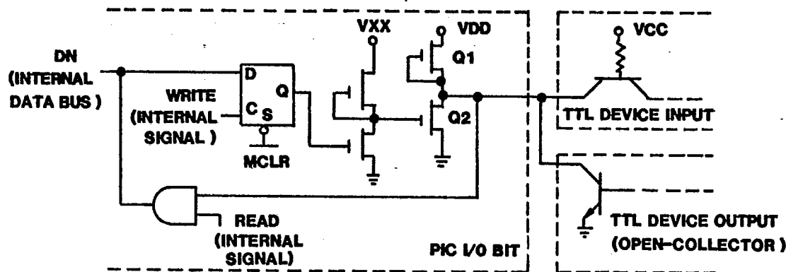
TYPICAL INTERFACE-BIDIRECTIONAL I/O LINE
