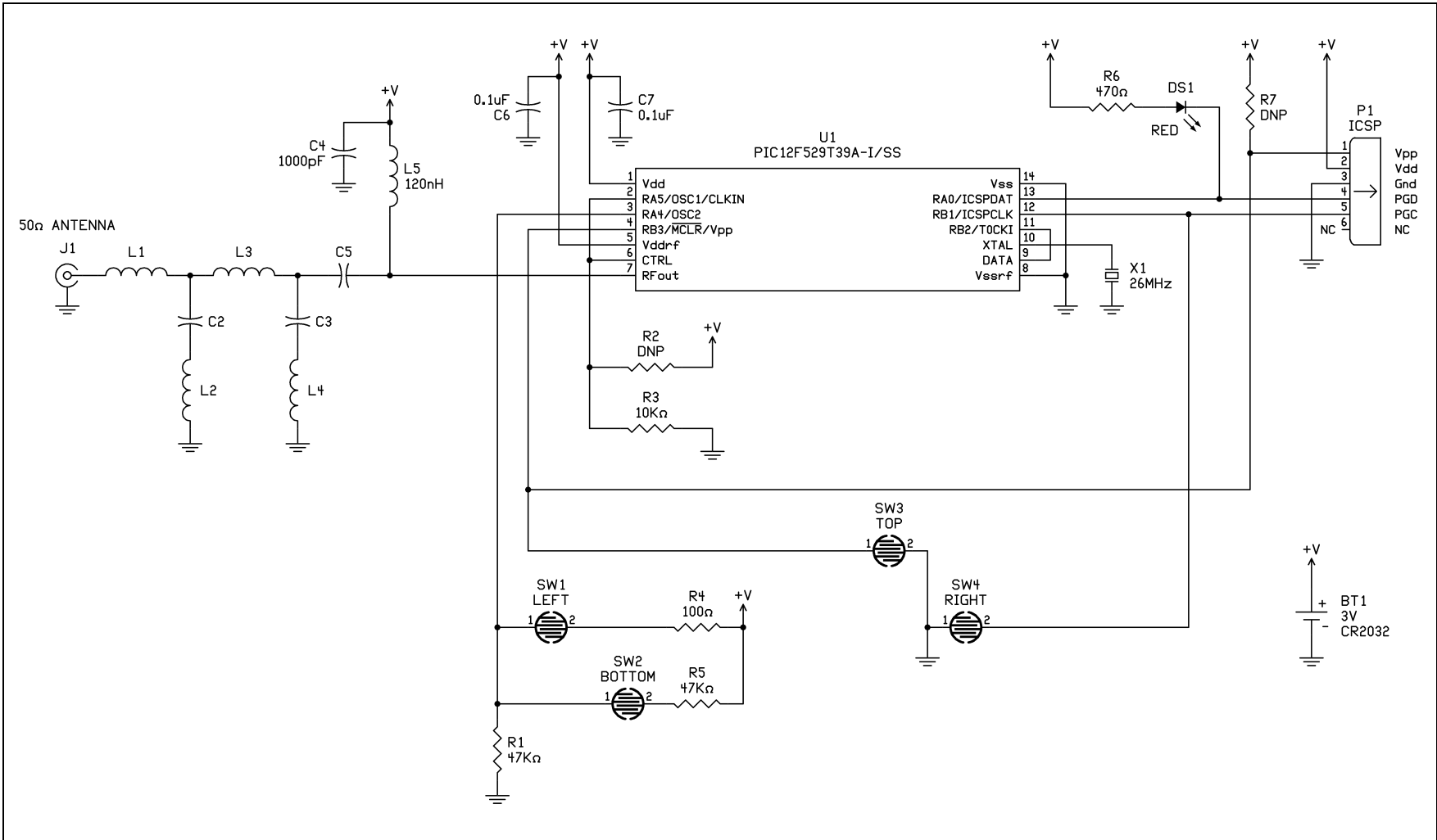
FIGURE 28-8: APPLICATION SCHEMATIC
