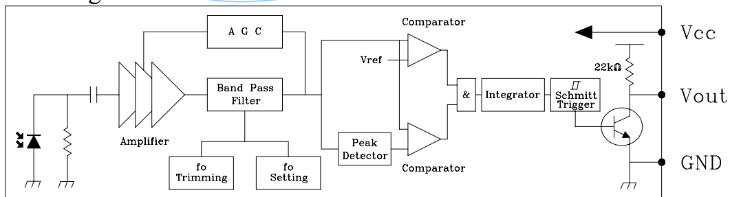
Block Diagram
