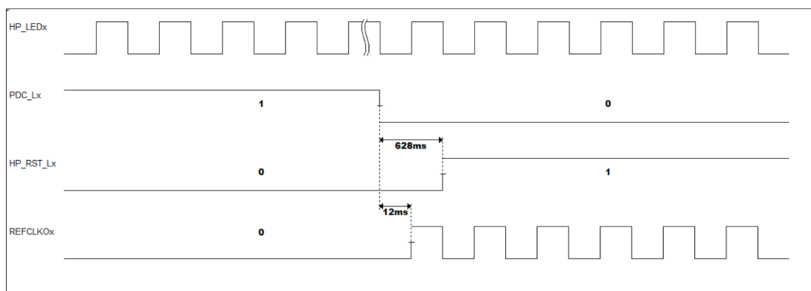
Figure 6-1 Timing Sequence for Surprised Hot Plug Insertion Operation
