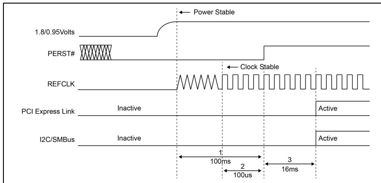
Figure 10-1 Initial Power-Up Sequence
