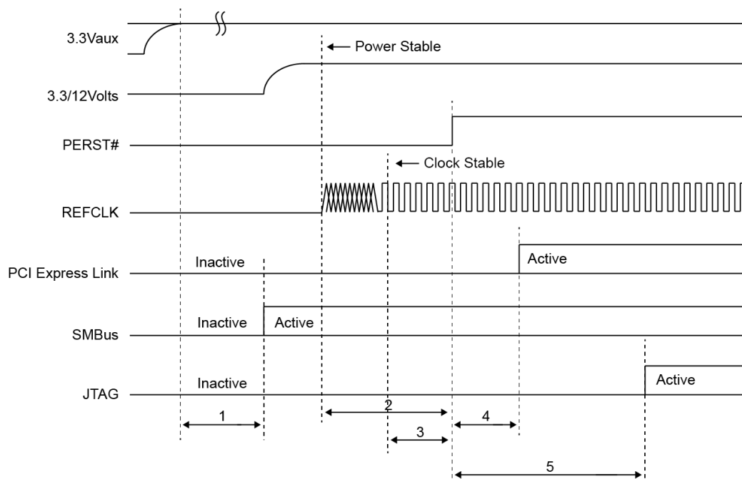
Figure 14-1 Initial Power-up
