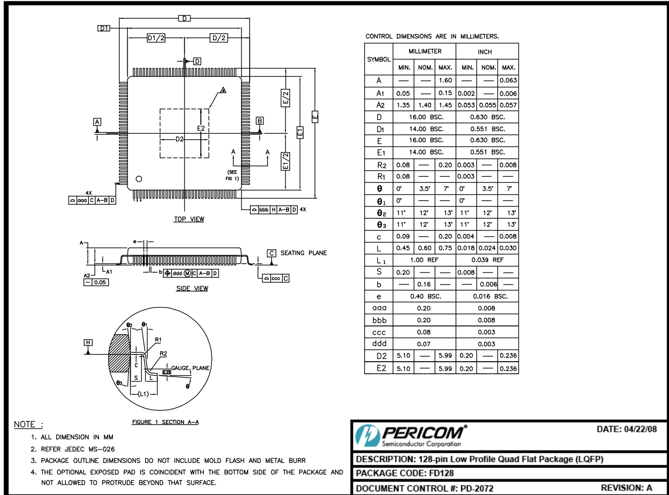
Figure 16-1 Package Outline Drawing
