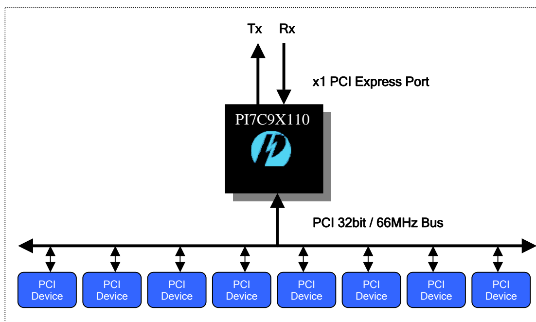
Figure 1-1 PI7C9X110 Topology
