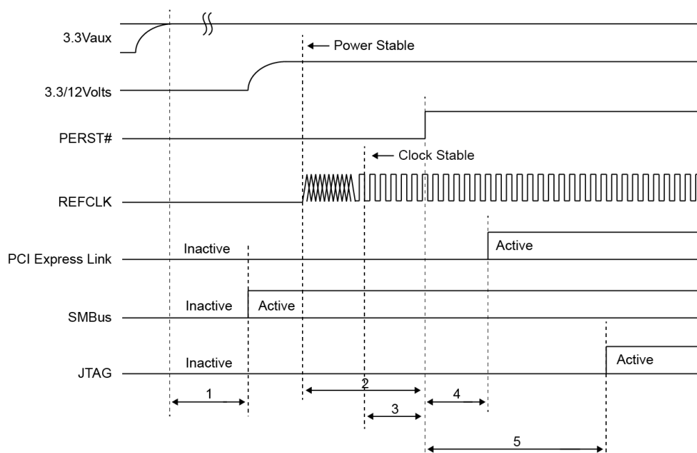
Figure 16-3 Initial Power-up
