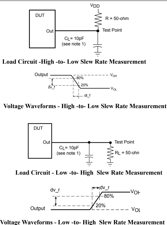
Figure 2. Output Slew-Rate Measurement Information ( V_{DD} = 1.8V \pm 0.1V )
