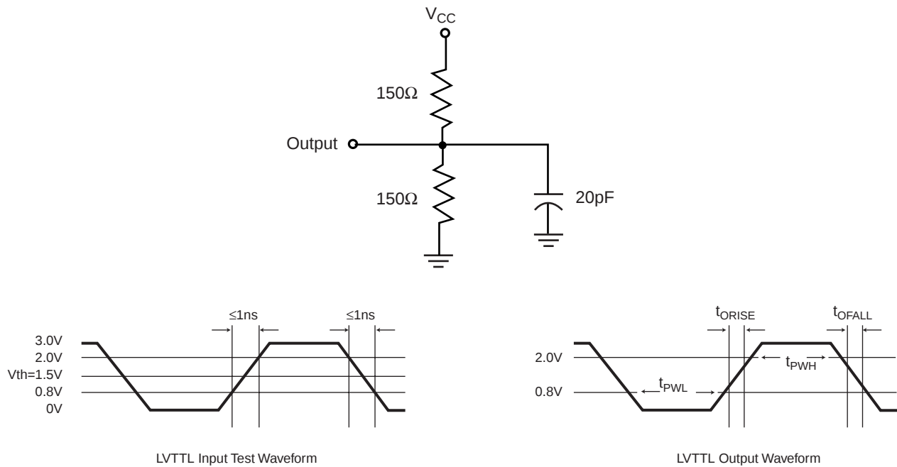
AC Test Loads and Waveforms
