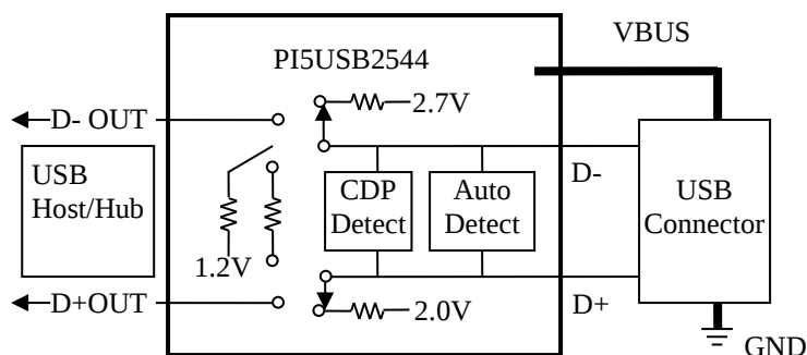
Figure 2a, Divider-1A Charging Scheme
