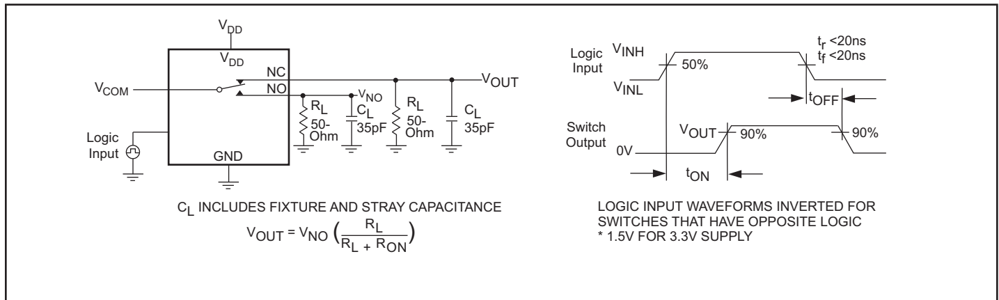
Figure 2. Switching Time
