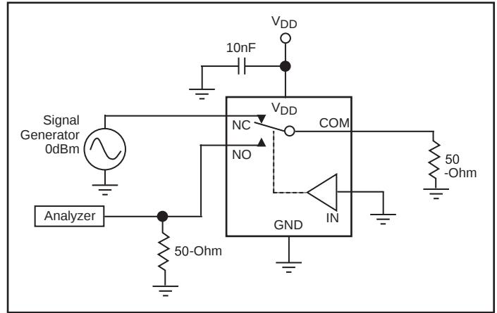
Figure 6. Crosstalk
