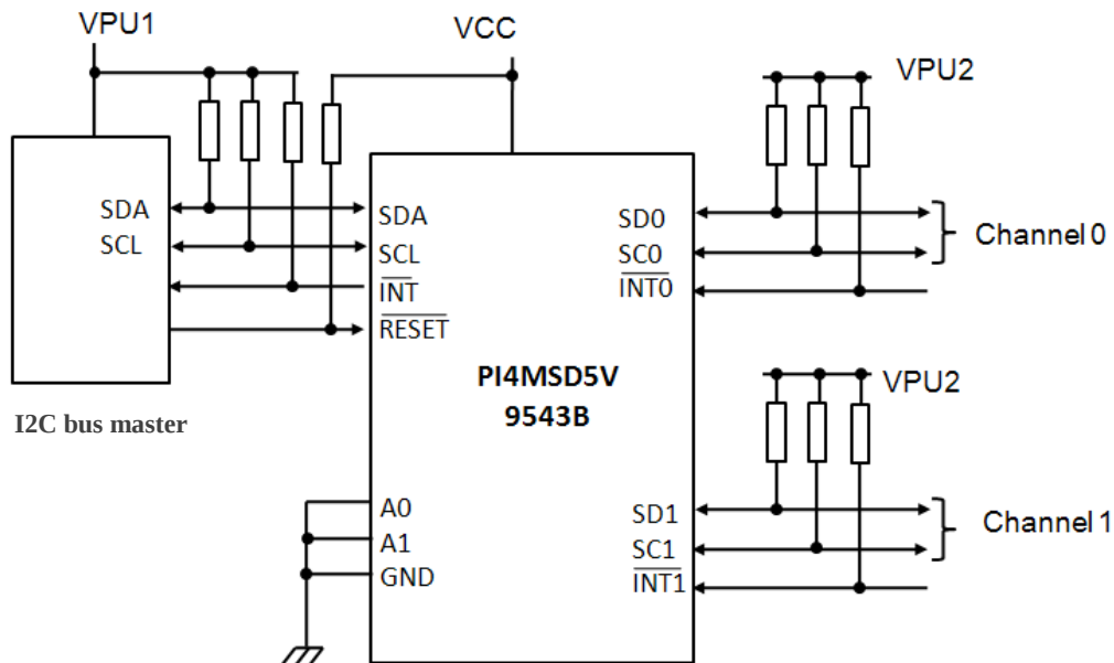
Figure 3. Typical Application
