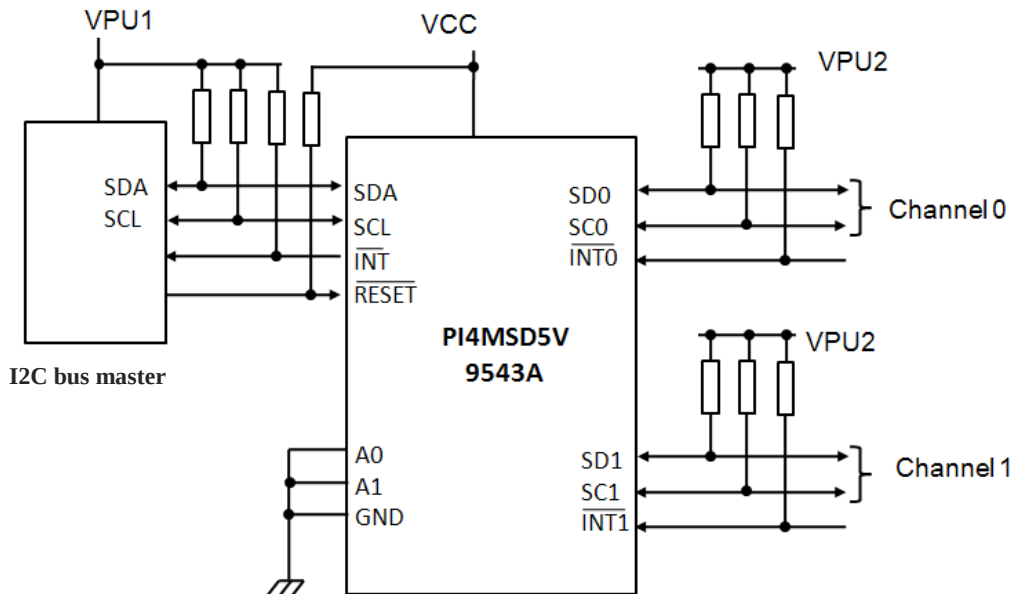
Figure 3. Typical Application
