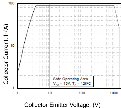
Figure 16. Turn-Off SOA
