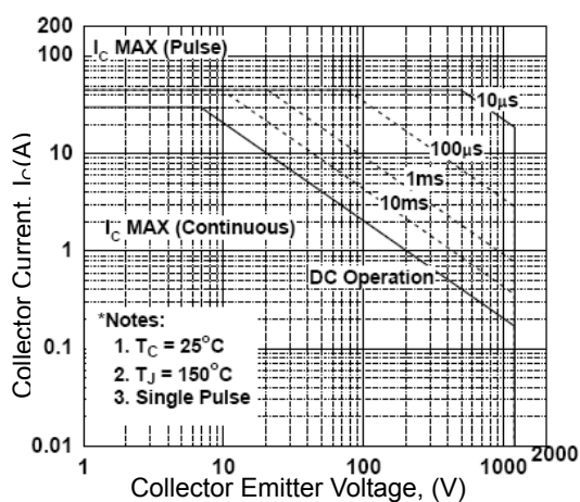
Figure 14. SOA Characteristics
