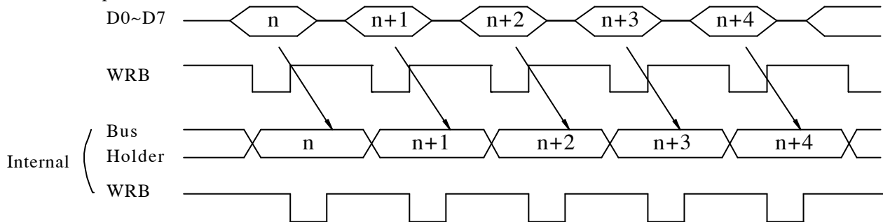
Data Write Operation
