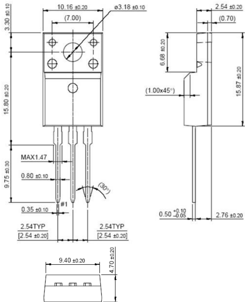
TO-220F (2)
