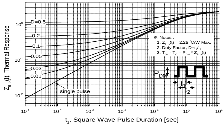
Figure 13. Transient Thermal Response Curve for PFF7N80
