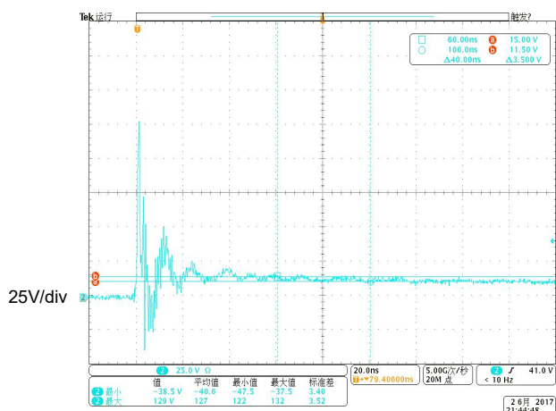
Fig 7. ESD clamping voltage (IEC61000-4-2 +8KV contact)
