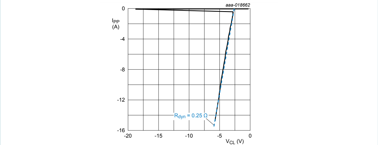
Fig. 5. Dynamic resistance with negative clamping voltage
