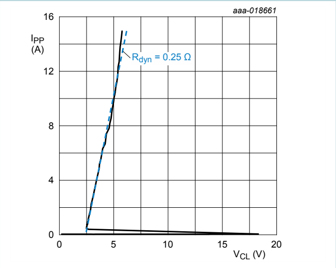
Fig. 4. Dynamic resistance with positive clamping voltage
