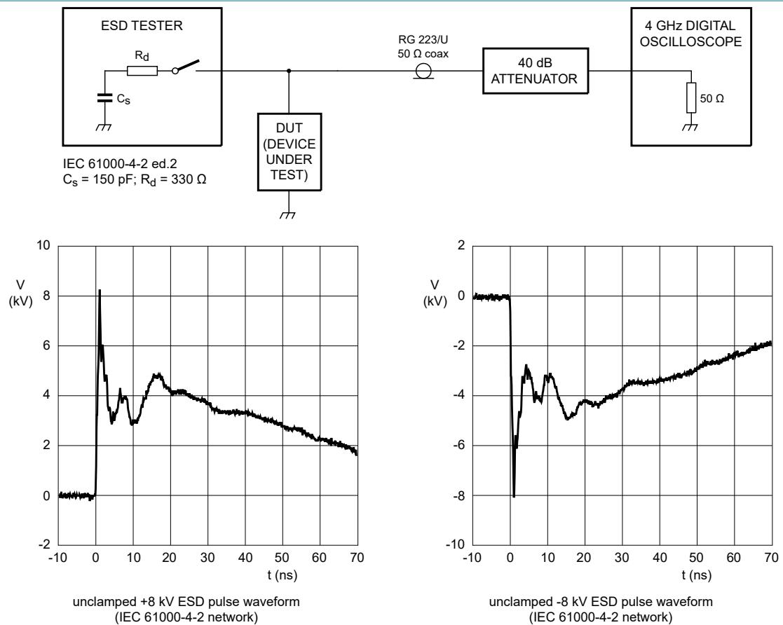
Fig. 6. ESD clamping test setup and waveforms
