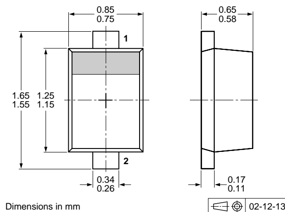
Fig 7. Package outline PESD3V3U1UB (SOD523/SC-79)
