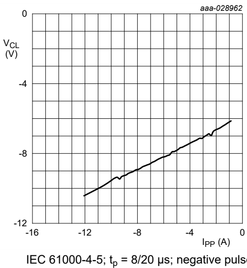
Fig. 9. Negative clamping voltage (8/20 \mu\text{s} pulse); typical values
