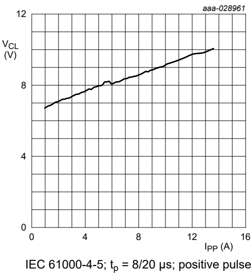
Fig. 8. Positive clamping voltage (8/20 \mu\text{s} pulse); typical values
