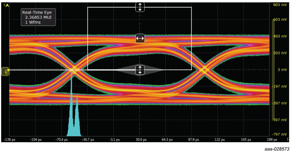
1080p, 6 Gbps Fig. 8. HDMI 2.0 eye diagram TP1, test board with PCMFxUSB3B/C; typical values
