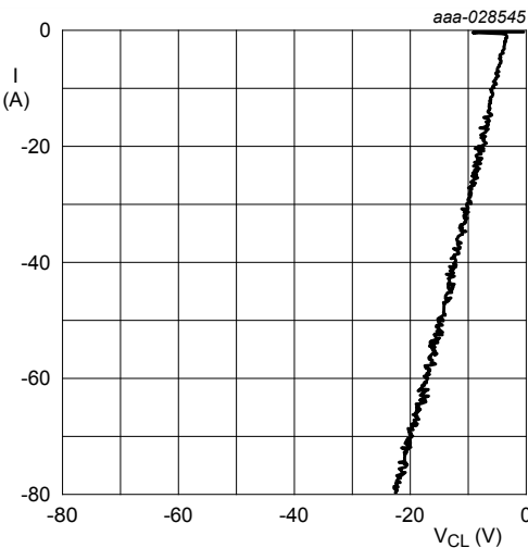
Fig. 15. Dynamic resistance with negative clamping; typical values
