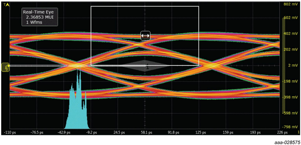
Fig. 10. HDMI 2.0 eye diagram TP2, test board with PCMFxUSB3B/C; typical values
