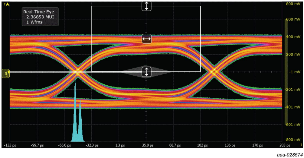
1080p, 6 Gbps Fig. 9. HDMI 2.0 eye diagram TP1, test board without device; typical values
