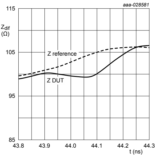
Fig. 3. Differential Time Domain Reflectometer (TDR) plot; typical values
