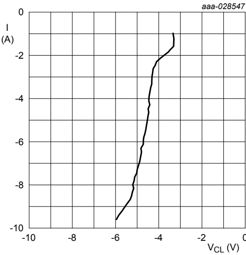
Fig. 17. Dynamic resistance with negative clamping; typical values
