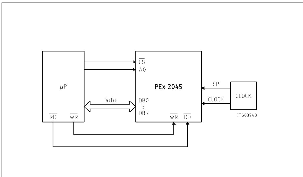
Figure 12 The PEx 2045 Controlled by a Microprocessor
