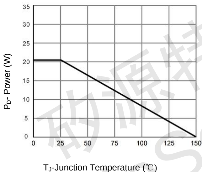
Figure 3 Power De-rating
