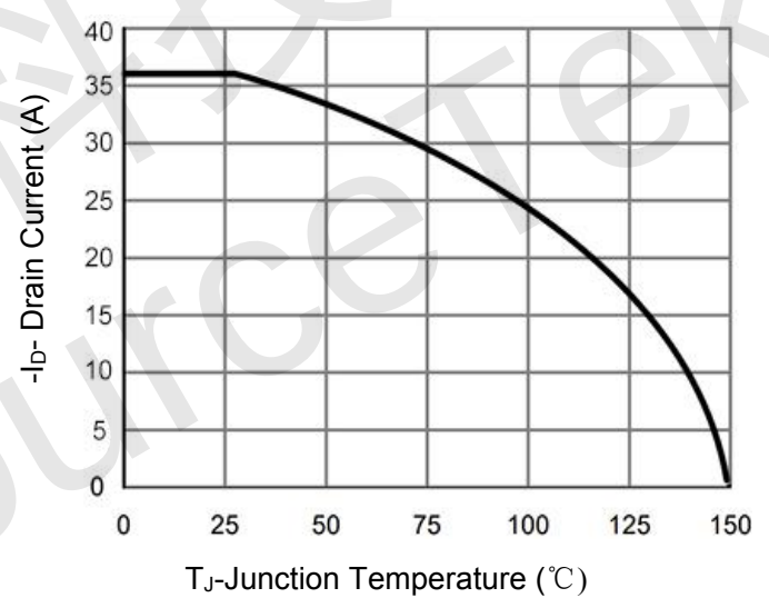
Figure 4 Drain Current
