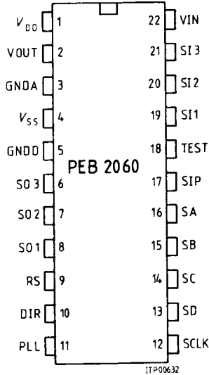
P-DIP-22
