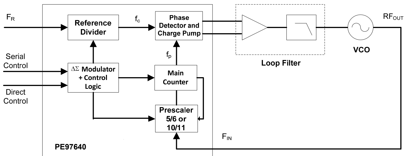
Figure 1. Functional Diagram
