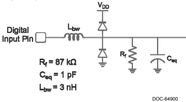
Figure 4. Equivalent Input Diagram: Digital Input
