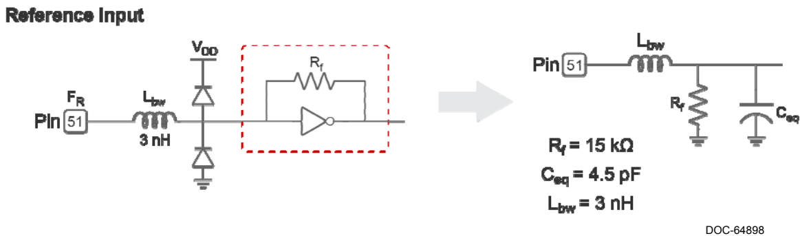
Figure 5. Equivalent Input Diagram: Reference Input
