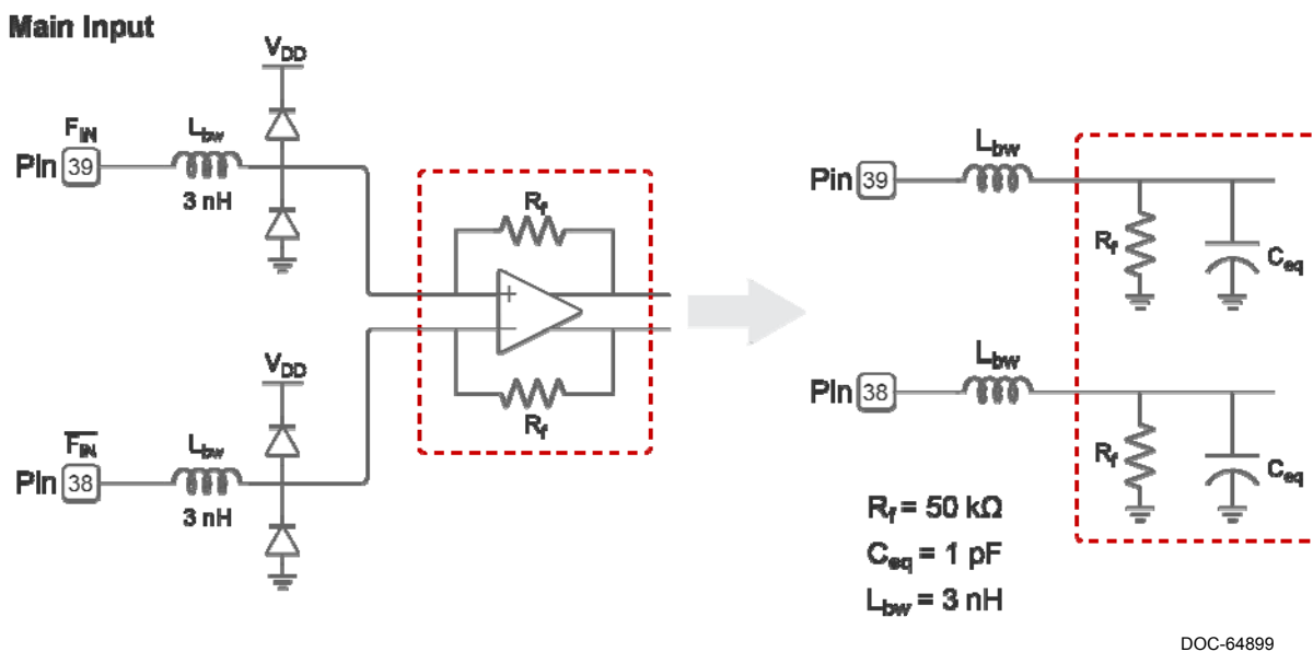
Figure 6: Equivalent Input Diagram: Main Input
