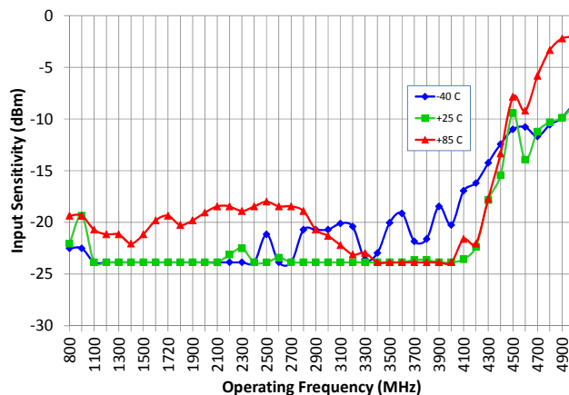
Figure 15. RF Sensitivity vs. F_{IN} and Temp (10/11 Prescaler, V_{DD} = 2.6\text{V} )*
