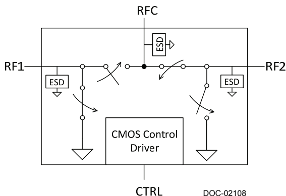
Figure 1. Functional Diagram
