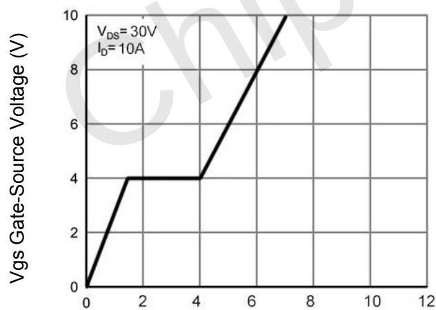
Figure 11 Gate Charge
