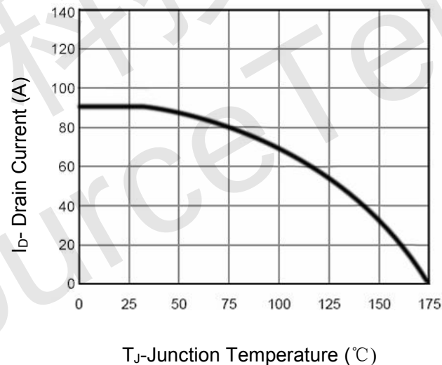
Figure 4 Drain Current
