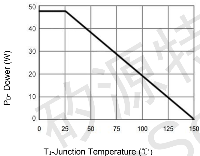
Figure 3 Power De-rating
