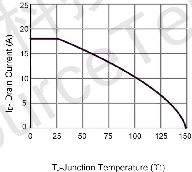
Figure 4 Drain Current
