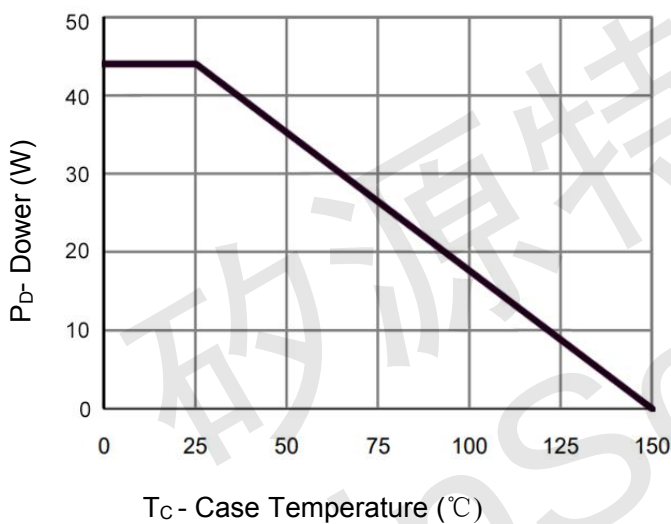
Figure 3 Power De-rating
