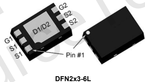
DFN2x3-6L
